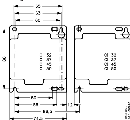
CI 32-50 with mechanical interlock Drilling dimensions
