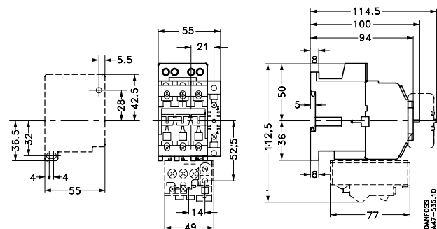
Contactors and motor starters CI 25EI, 30 EI, 25DC, 30DC
