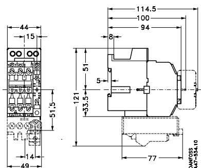
Contactors and motor starters CI 9EI, 15EI, 9DC, 15DC
