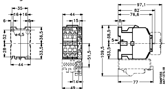
Control relays, contactors and motor starters, CI 6, 9, 12, 15 Drilling dimensions
